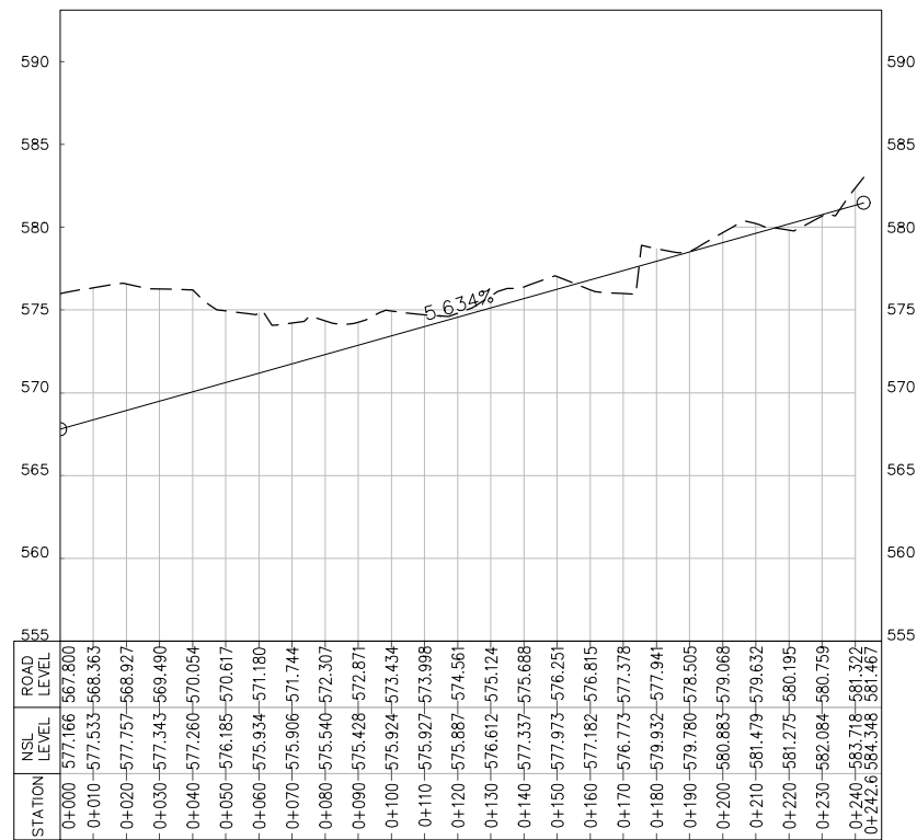
OUTLET ACCESS ROAD PROFILE SCALE B
