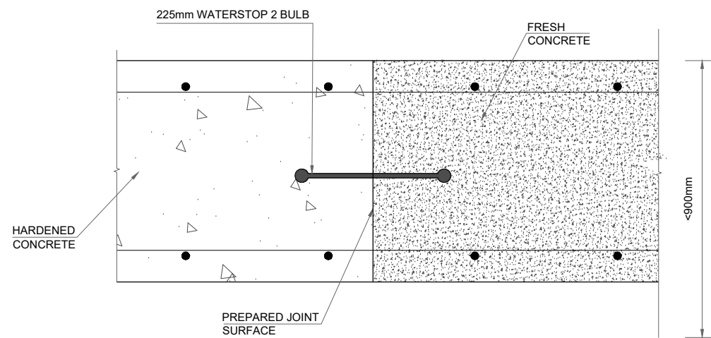
CONSTRUCTION JOINT IF THICKNESS IS LESS THAN 900 mm
