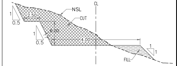
TYPICAL SECTION
