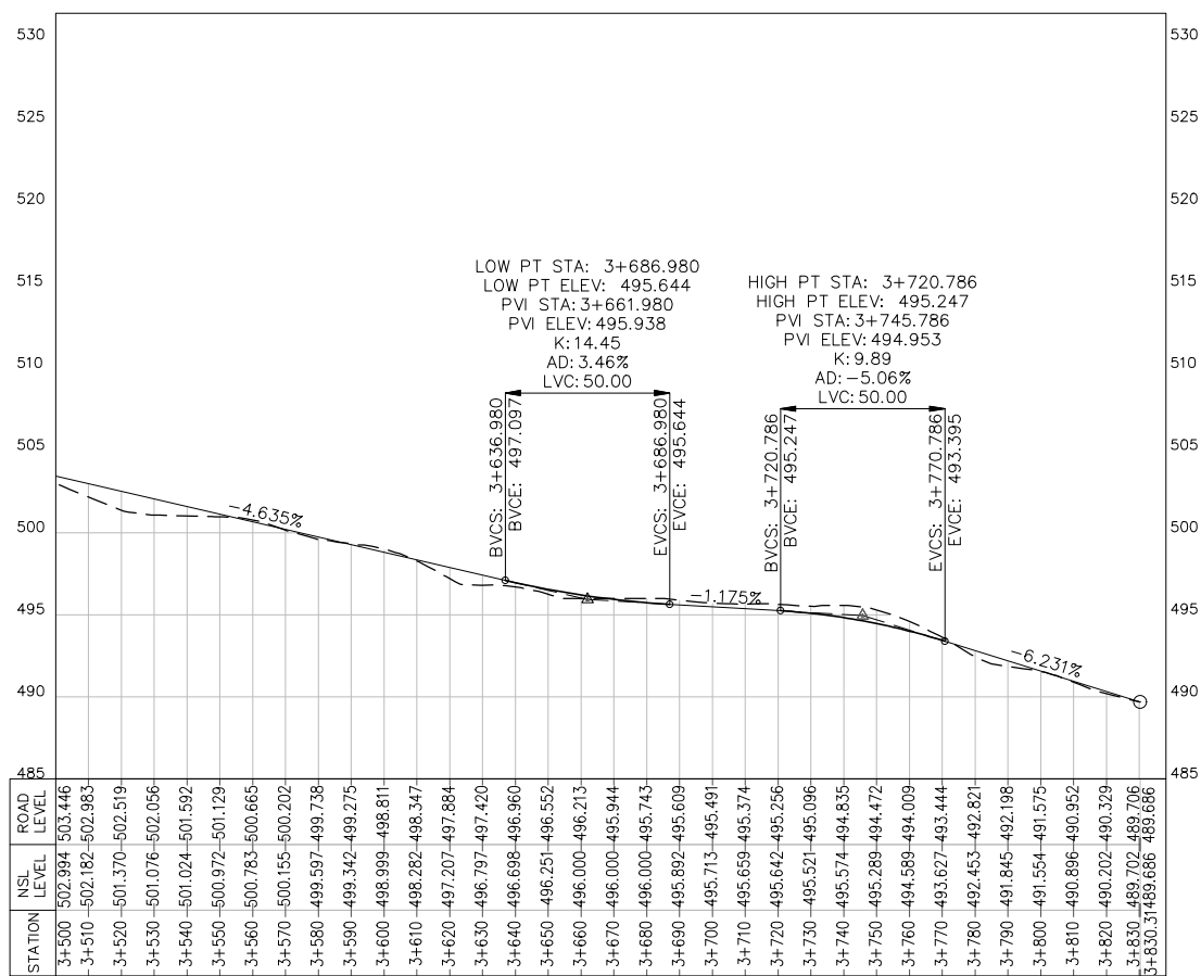
PROFILE SCALE B
