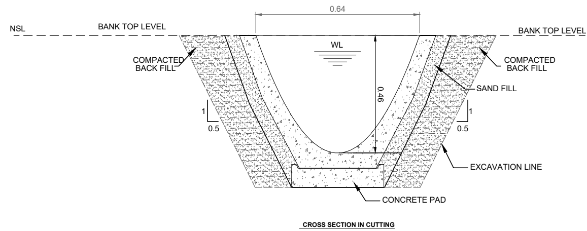
CROSS SECTION IN CUTTING
