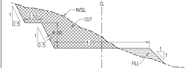
TYPICAL SECTION
