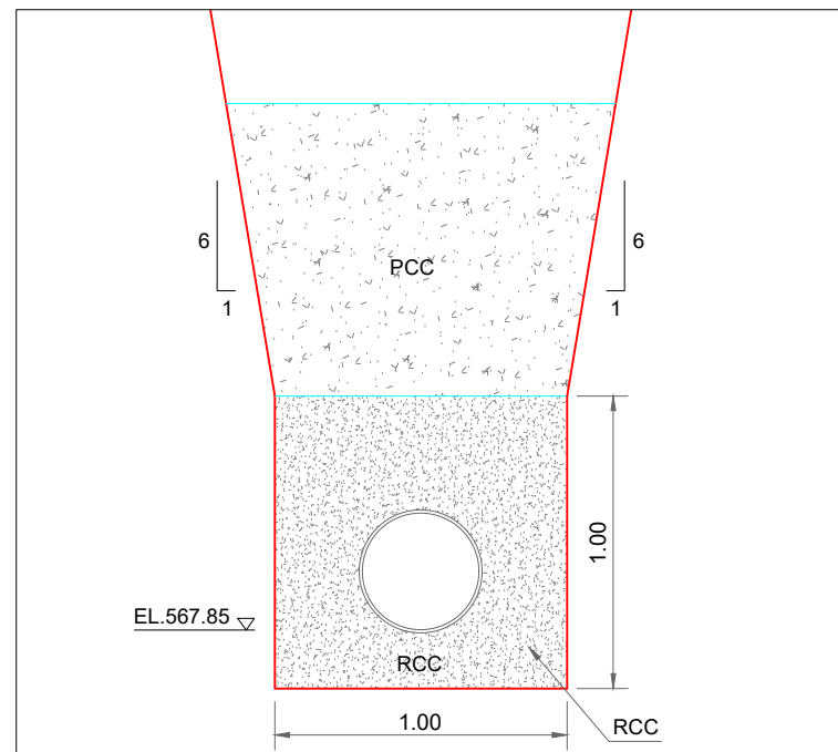
DETAIL "A"
