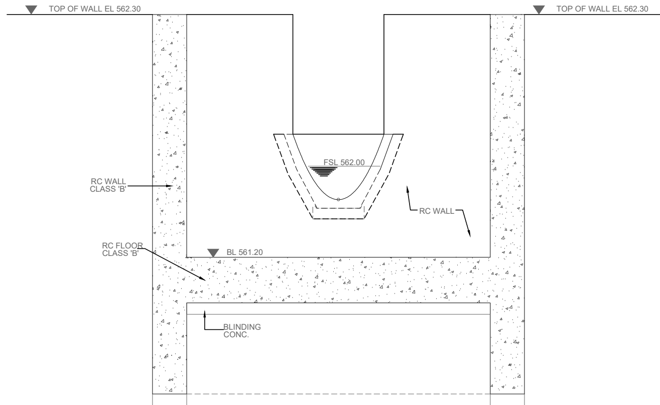
SECTION E-E
