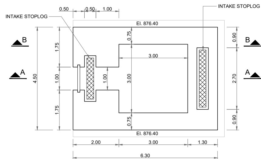
SECTION D-D AT EL.880.00
