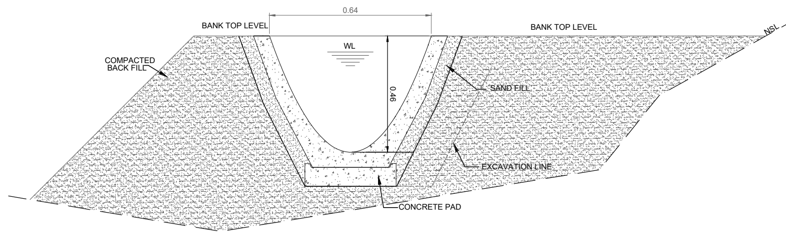
CROSS SECTION IN FILLING
