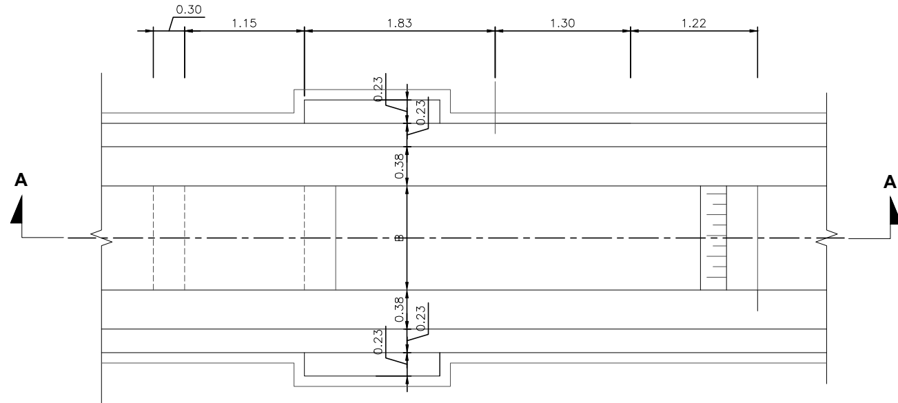
TYPICAL CANAL FALL PLAN
