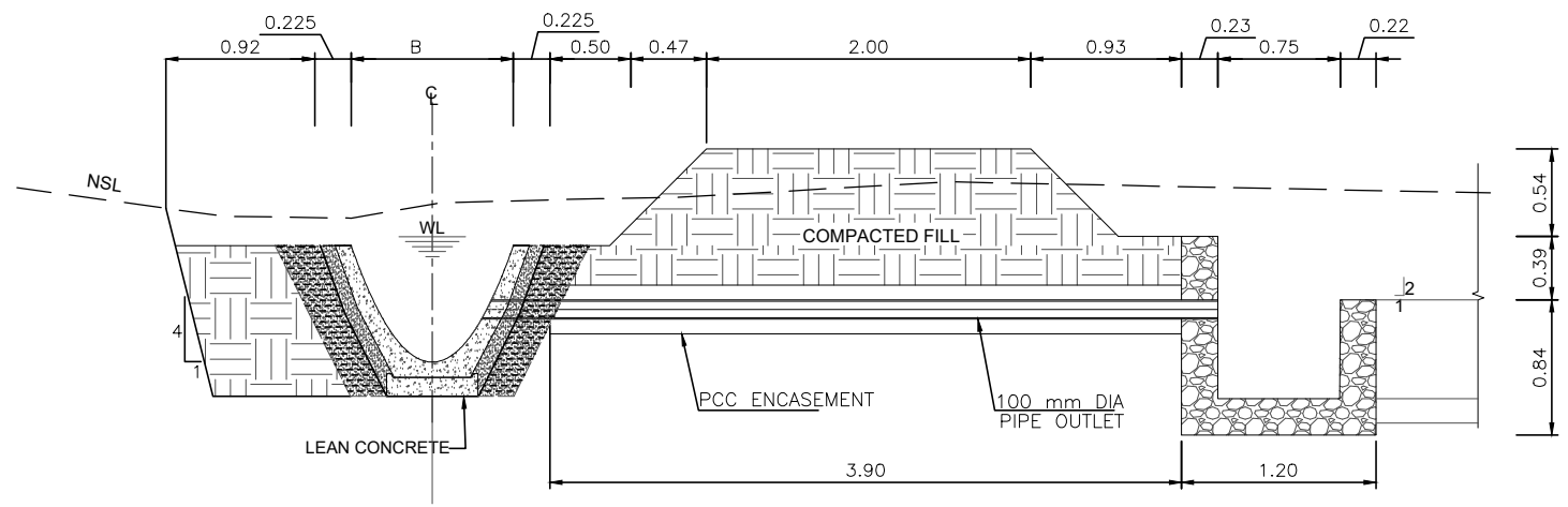
TYPICAL PIPE OUTLET CROSS SECTION B-B
