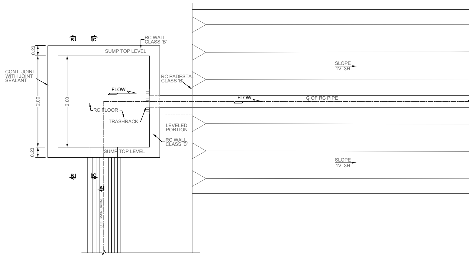
U/S PART PLAN
