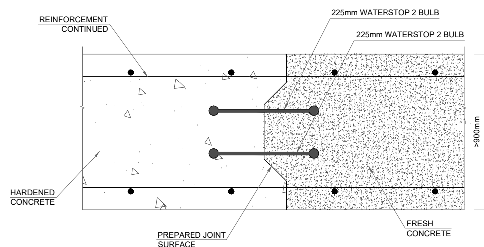
CONSTRUCTION JOINT IF THICKNESS IS GREATER THAN 900 mm
