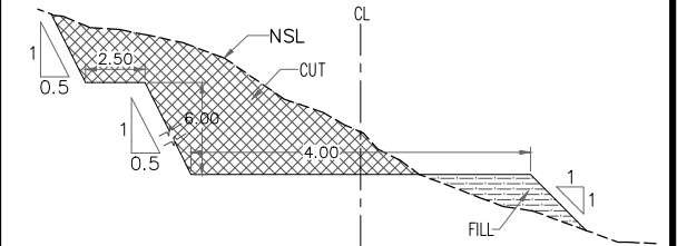
TYPICAL SECTION
