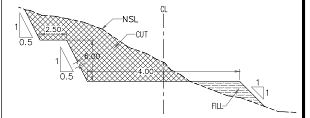
TYPICAL SECTION
