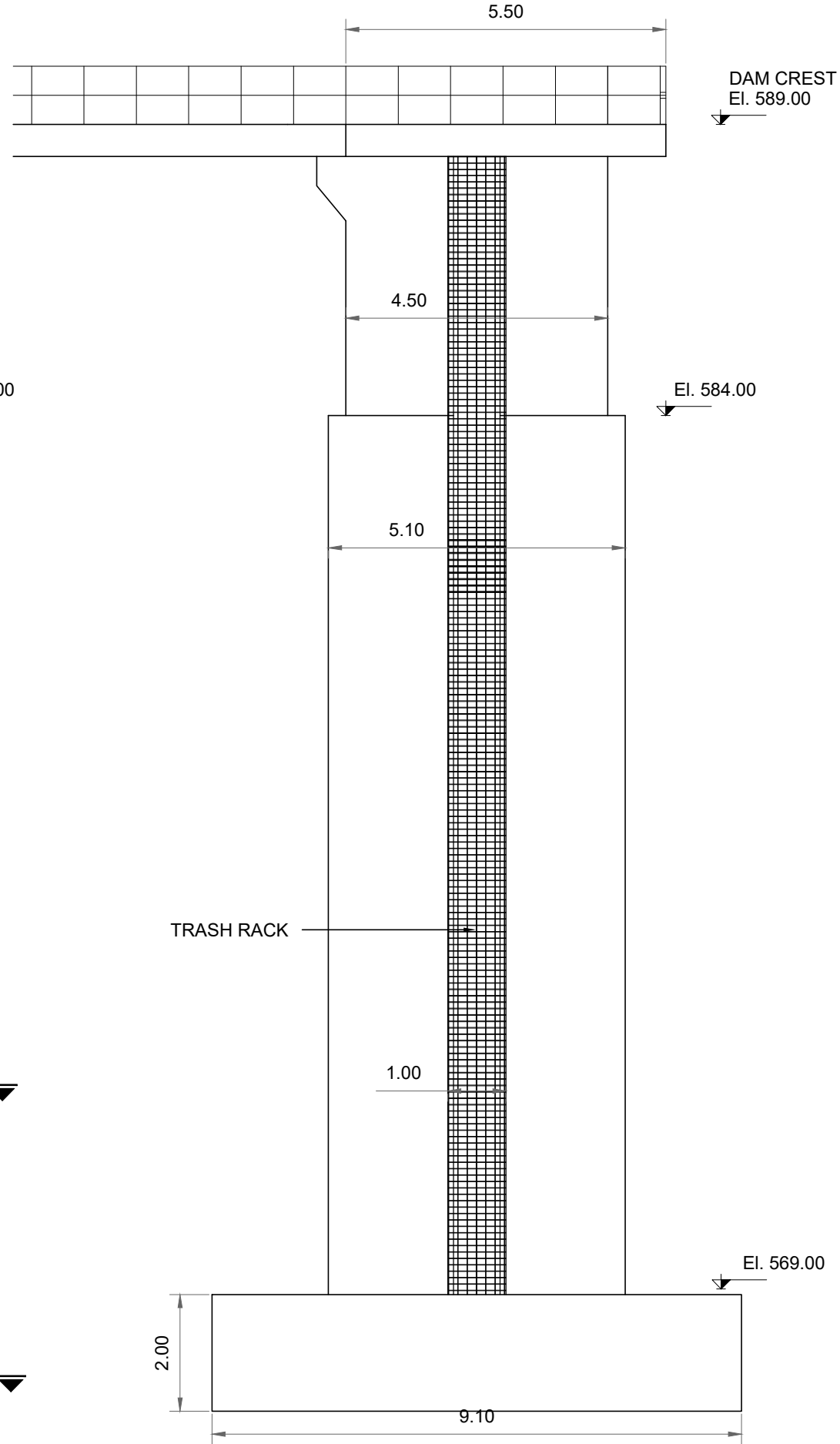
FRONT VIEW
