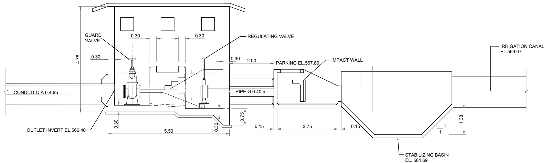
OUTLET STRUCTURE SECTION
