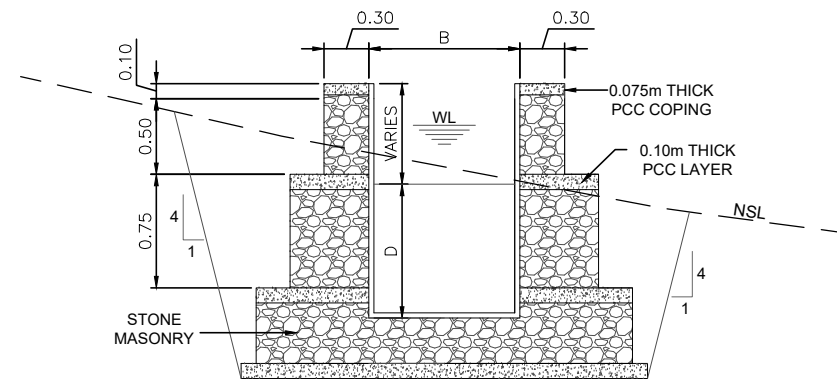
CANAL FALL CROSS SECTION B-B
